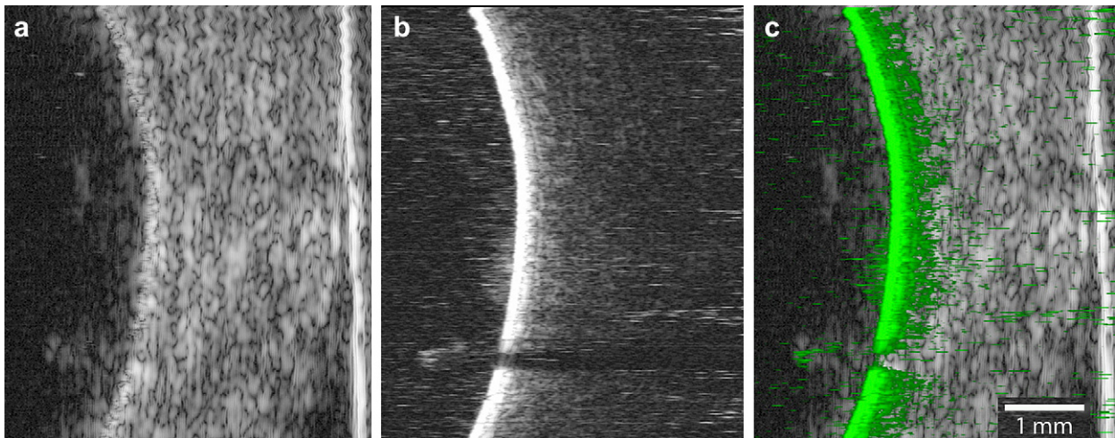
Fig. 7. Pulse/echo (a) and photoacoustic (b) images of the choroid in an ex vivo pig eye obtained with the 20-MHz ring transducer using a 532-nm green laser. In pulse/echo mode, the choroidal surface and underlying sclera all produce echoes. In the photoacoustic image, a large signal is generated at the choroidal surface. Note the shadow from debris anterior to the choroidal surface (possibly detached retina). Acoustic signals appear in the photoacoustic image several microseconds after encountering strong absorbance by the choroid. In (c), the photoacoustic data (rendered in green) are superimposed on the gray-scale pulse/echo data to form a fused image.
