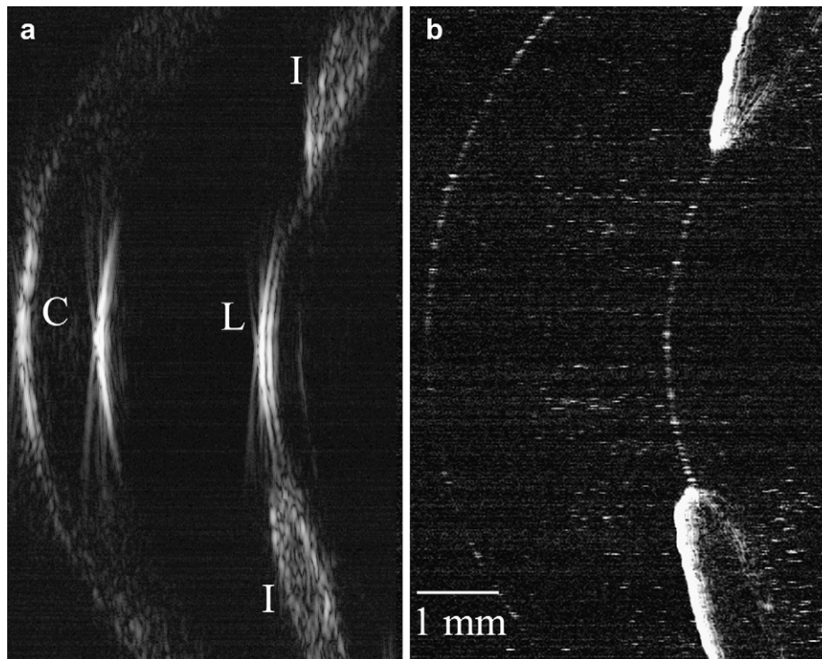
Fig. 5. Pulse/echo (a) and 532-nm photoacoustic image (b) of anterior segment of ex vivo pig eye obtained using 20-MHz probe with coaxial optics. The pulse/echo image shows reflections from the specular corneal (C) surfaces and that of the lens (L), as well as backscatter from the iris (I). The pigmented iris absorbs light and hence is visible photoacoustically. The anterior surfaces of the cornea and the lens both produce photoacoustic signals. Also present in the photoacoustic image are semi-random signals appearing a few microseconds after large acoustic emissions, possibly due to collapse of microbubbles.
